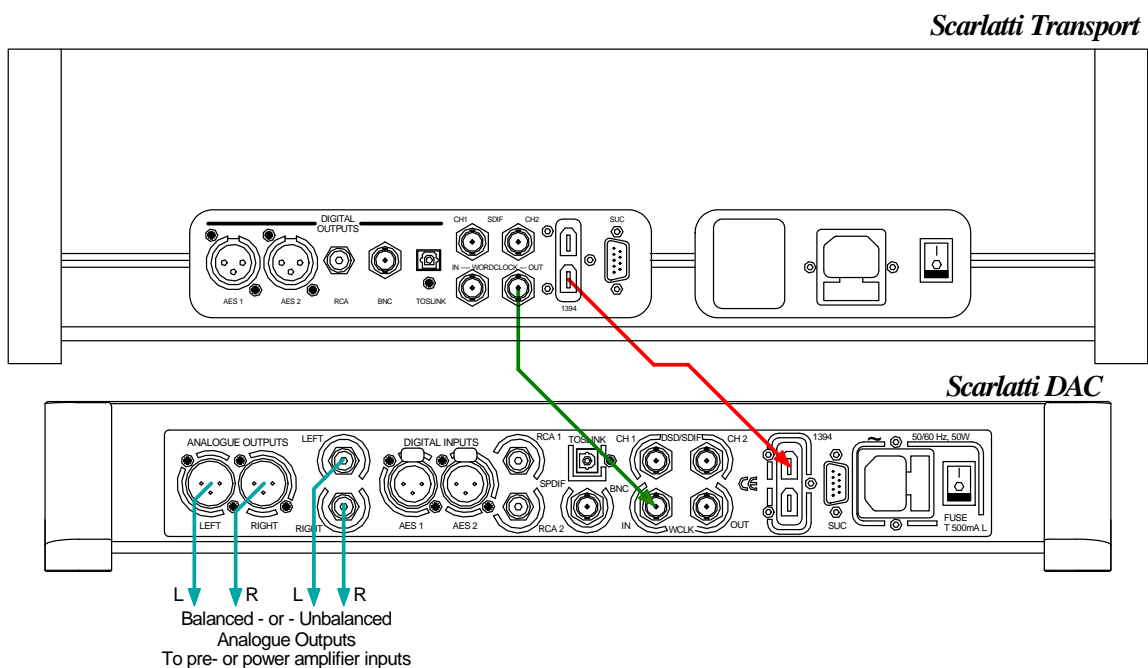
Figure 1 – Basic setup
