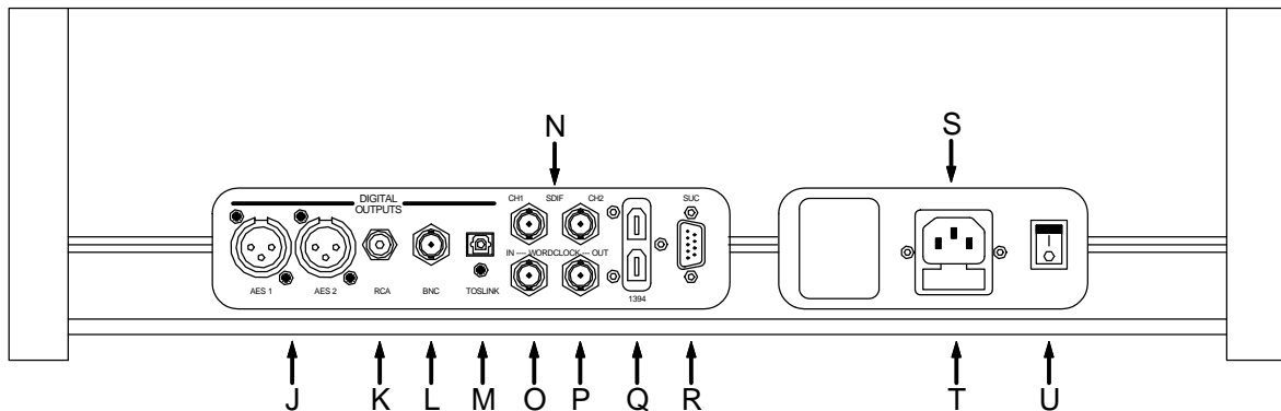
Figure 5 – Rear panel
