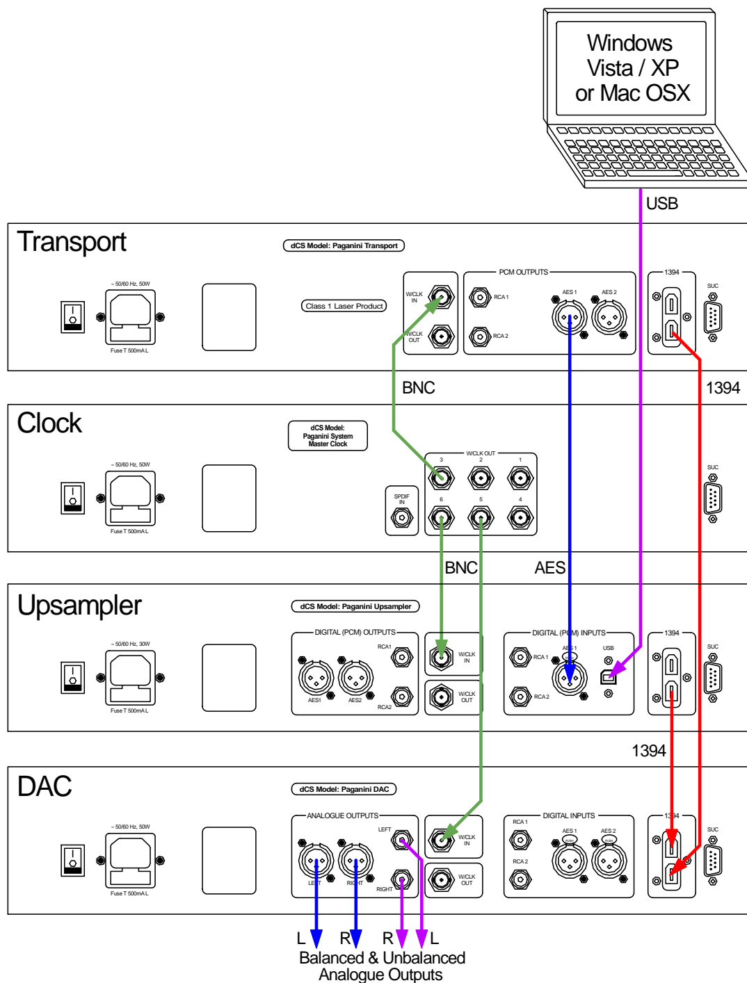
Figure 4 – An example of a full Paganini system plus a laptop
